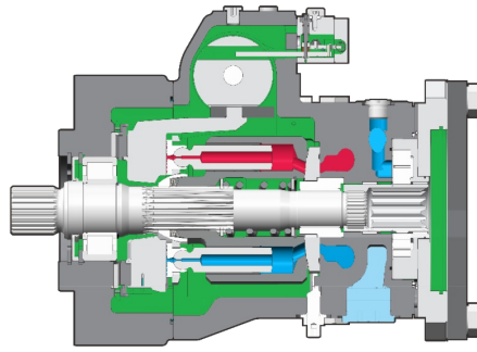
HP4G175 half-section diagram
